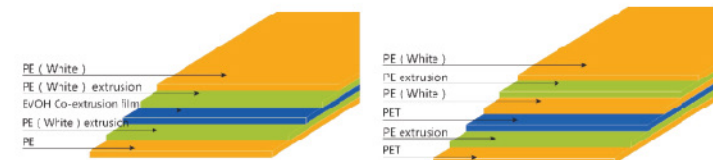
White/Clear Plastic Sheet with EVOH (thickness 330.370 μm)
